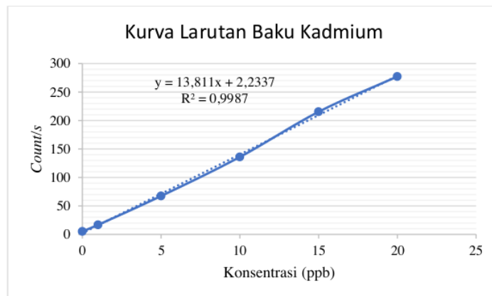
Gambar 1. Kurva Larutan Baku Kadmium
